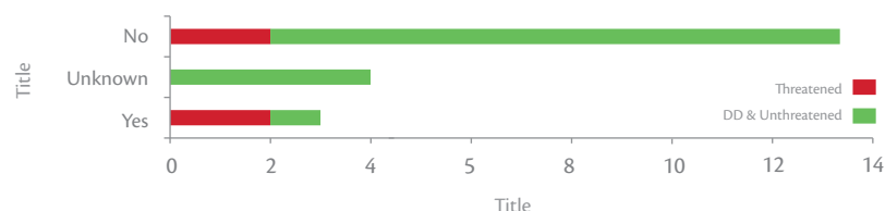
Figure 22: Occurrence of marine mammal species in at least one PA.
